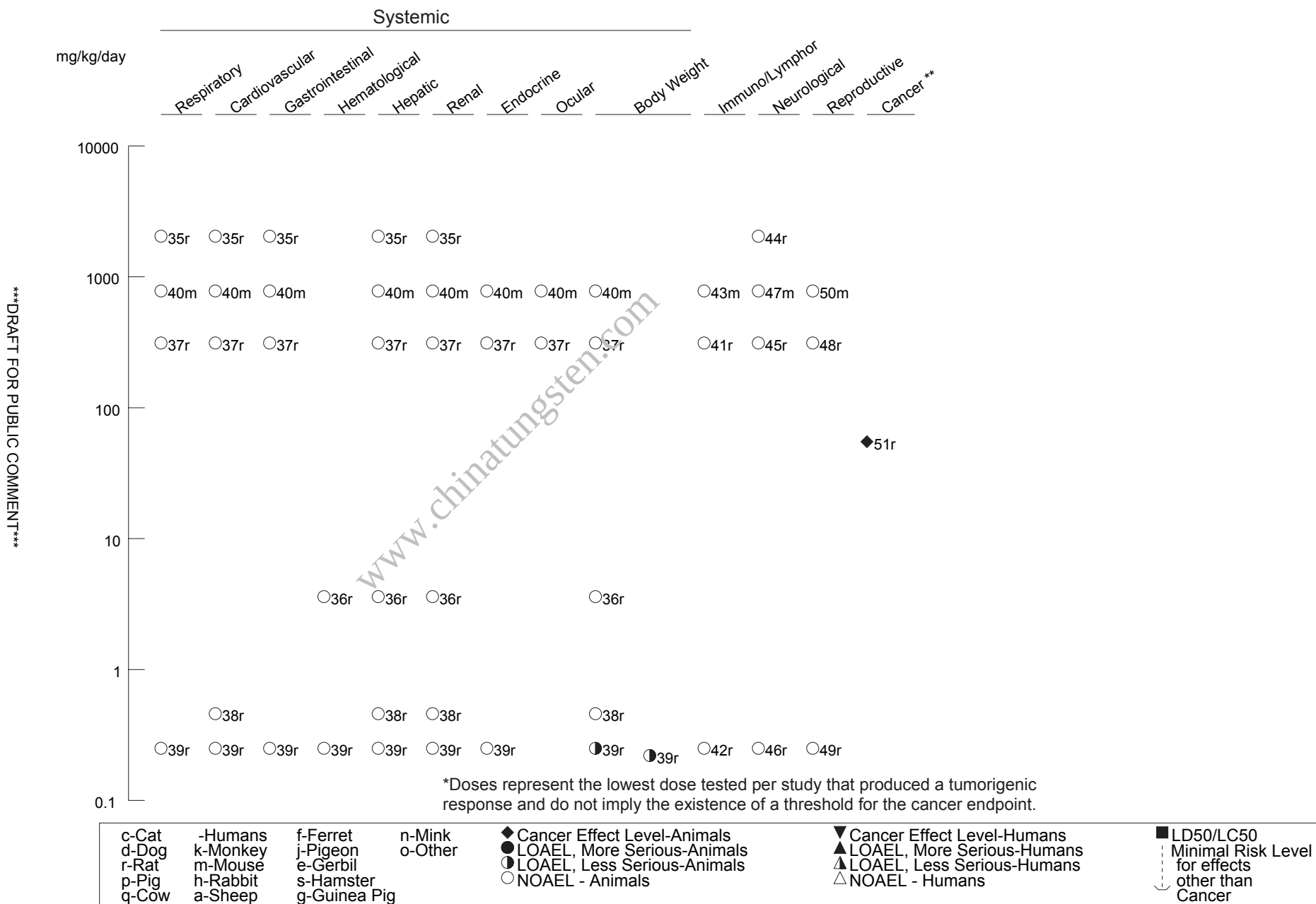
Figure 3-4 Levels of Significant Exposure to Chromium III - Oral (Continued)
