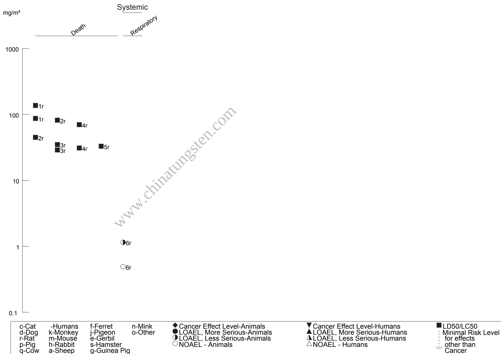
Figure 3-1 Levels of Significant Exposure to Chromium VI - Inhalation Acute ( \leq 14 days)
