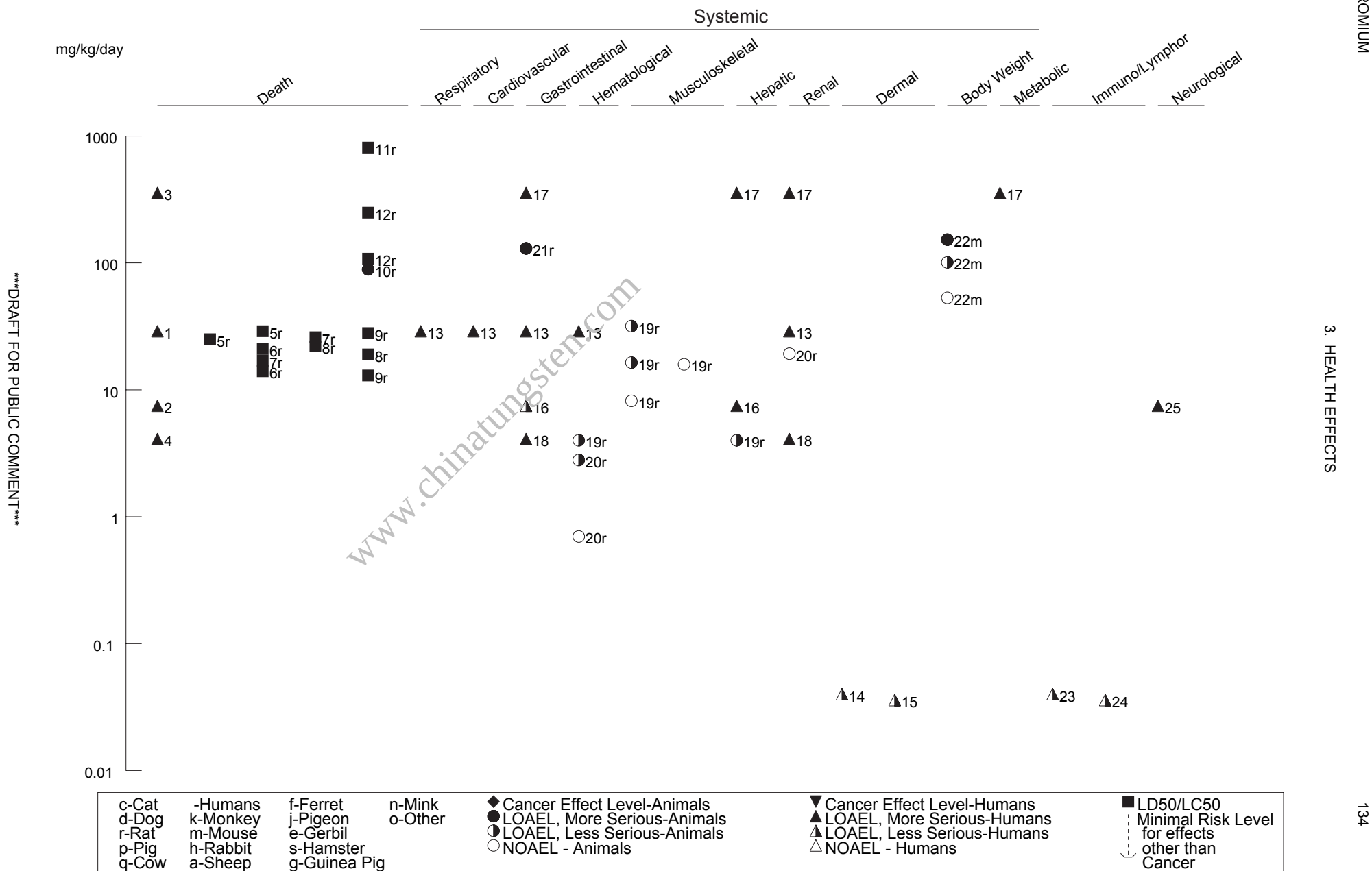
Figure 3-3 Levels of Significant Exposure to Chromium VI - Oral Acute (≤14 days)
